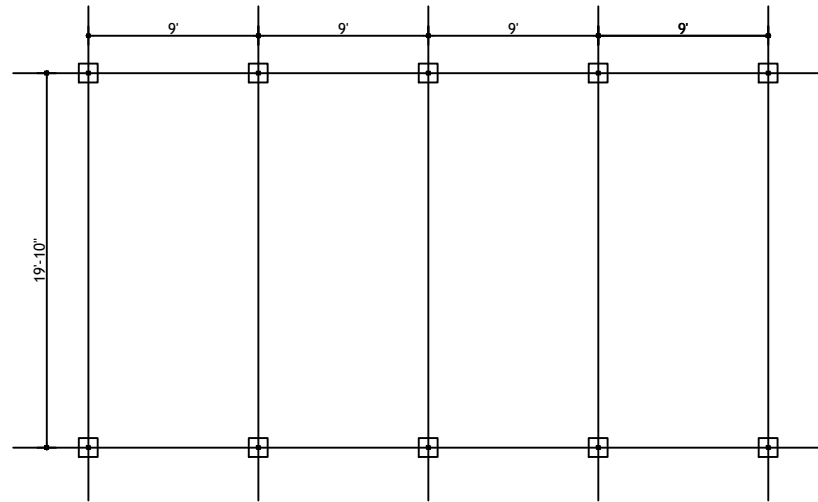
TRENCH PLAN
