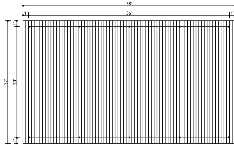
ROOF PLAN
