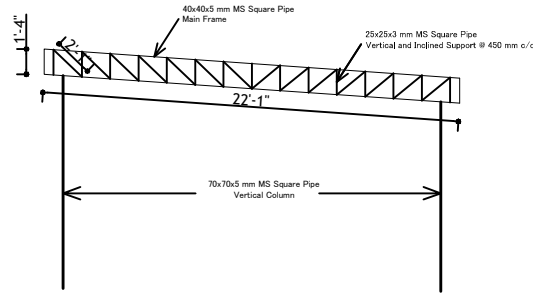
TRUSS DETAIL
